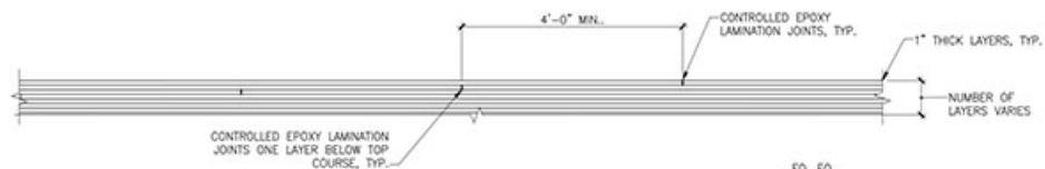
ELEVATION VIEW A-A
