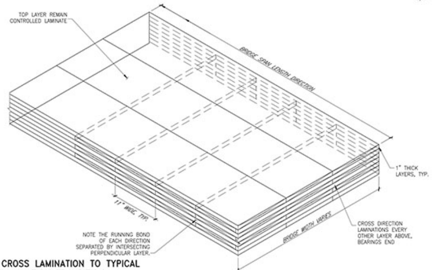
2 CROSS LAMINATION TO TYPICAL LAMINATION TRANSITION
