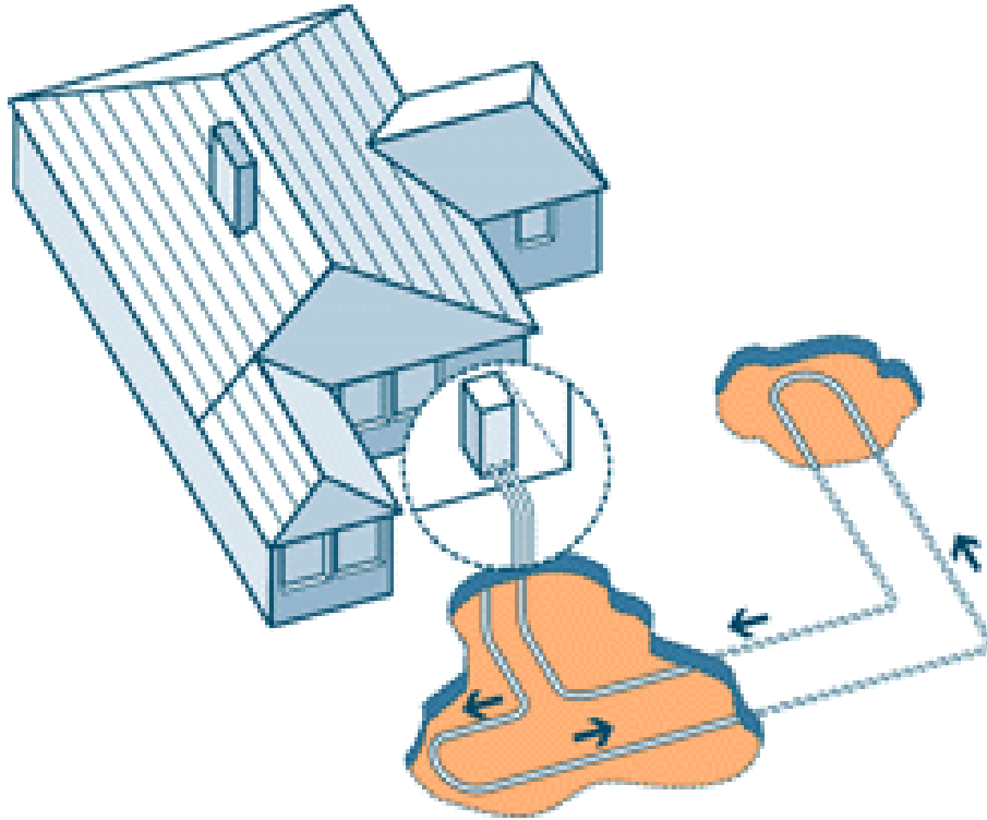
Closed-Loop, Single Layer Horizontal Configuration
