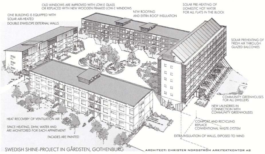
Top: birdview of one of three similar blocks describing the solar- and sustainable technologies.
