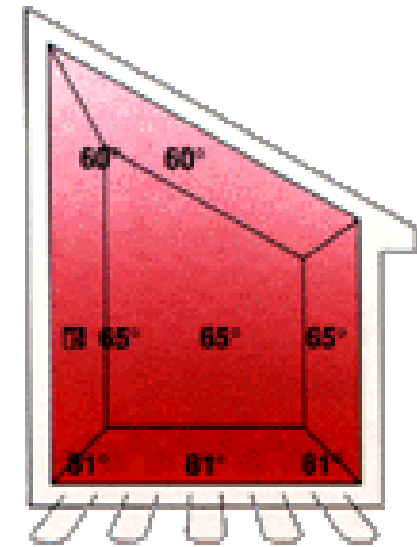
Radiant Floor
