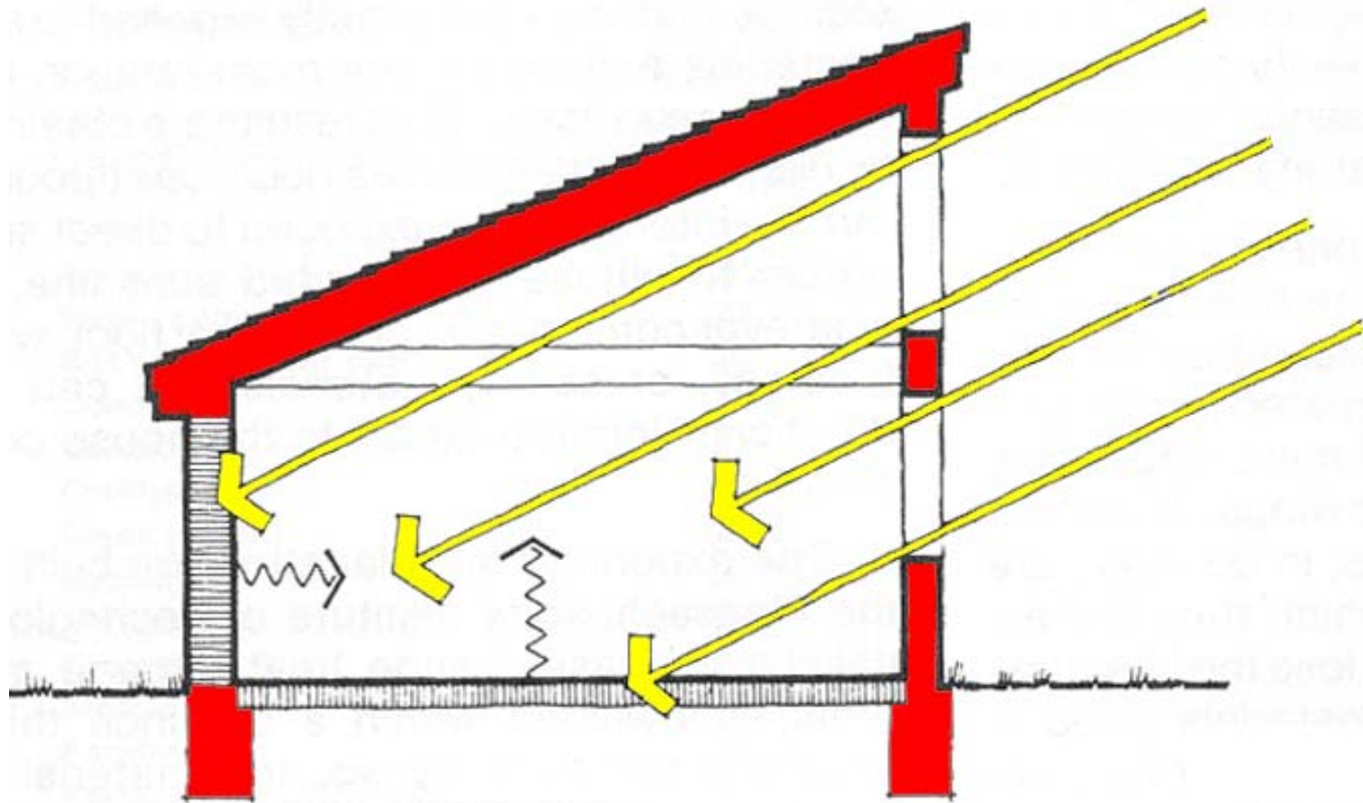
FIG. 19a. Direct Gain
