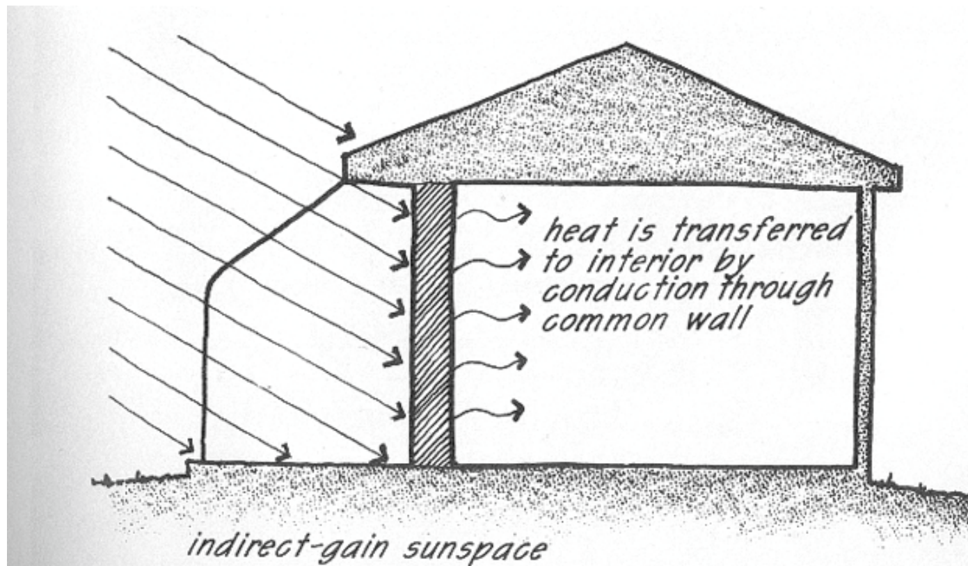
Figure 10.1: Indirect-gain sunspace building with common thermal storage wall. Conduction through the common wall is the primary means of heat transfer to living space.
