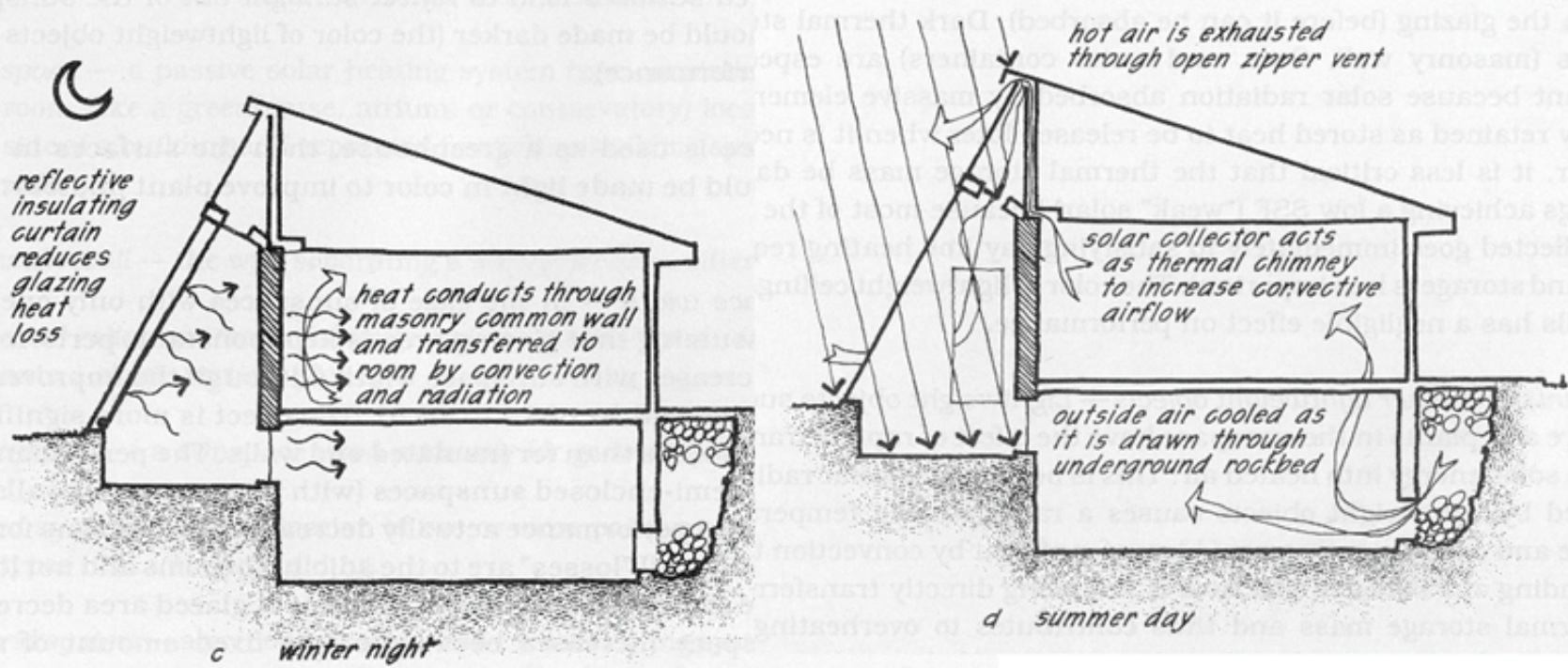
Figure 10.9 (continued): Solargreen passive operation: (c) winter night, and (d) summer day.
