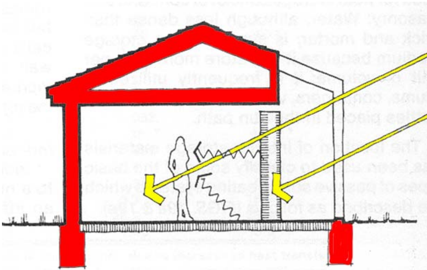
FIG. 19b. Direct and Indirect Gain
