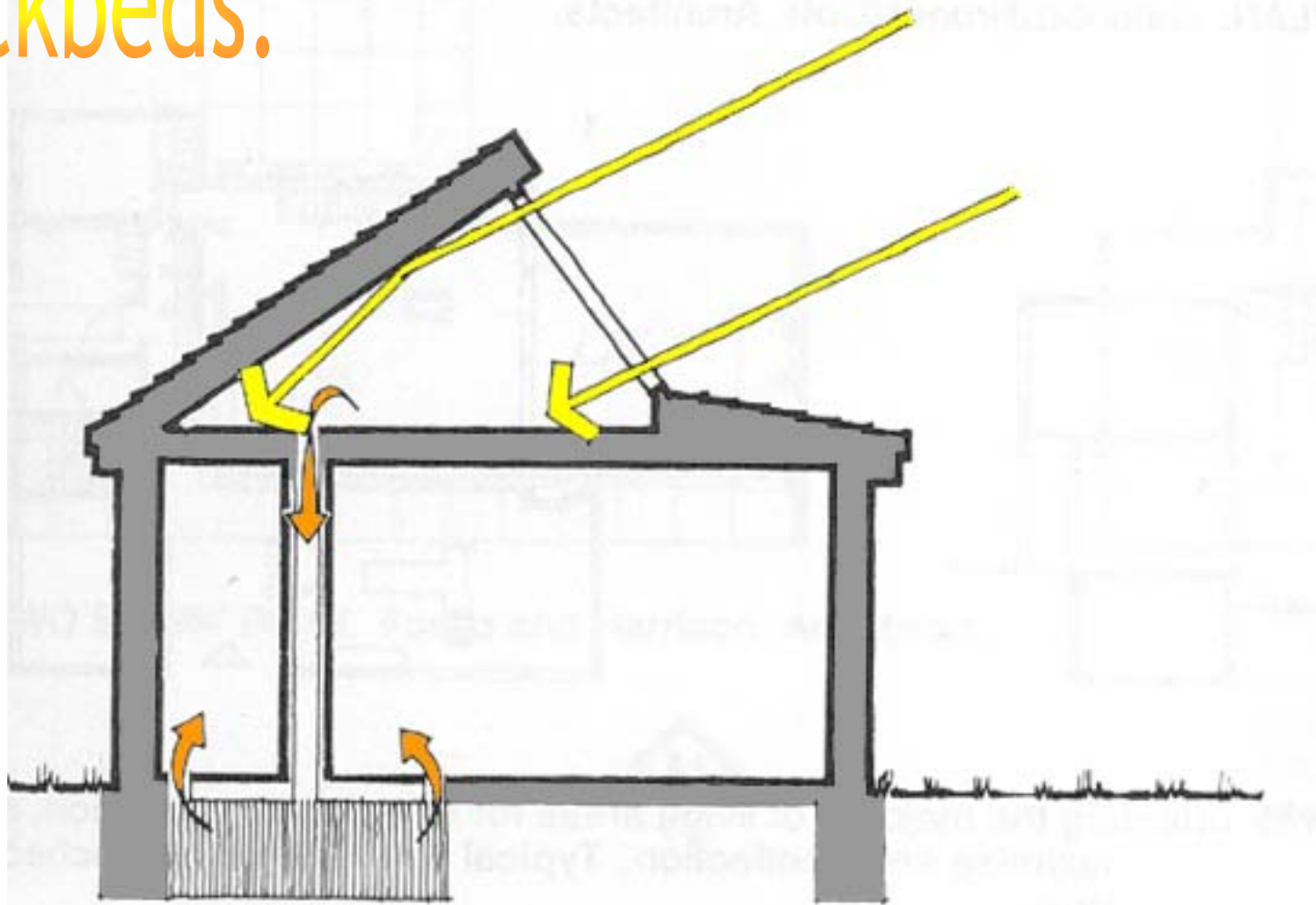
FIG. 19e. Remote Gain and Storage
