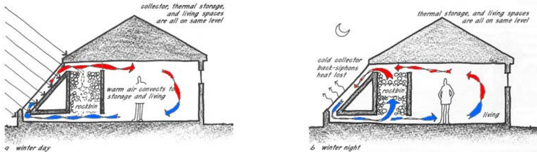
Figure 11.1: Positioning the collector, storage, and living areas at the same level in a convective air loop system: (a) winter day operation — level arrangement allows convective heating to occur during the day; (b) winter night operation — this "level" positioning of components permits unwanted back-siphoning, effectively cooling the system.
