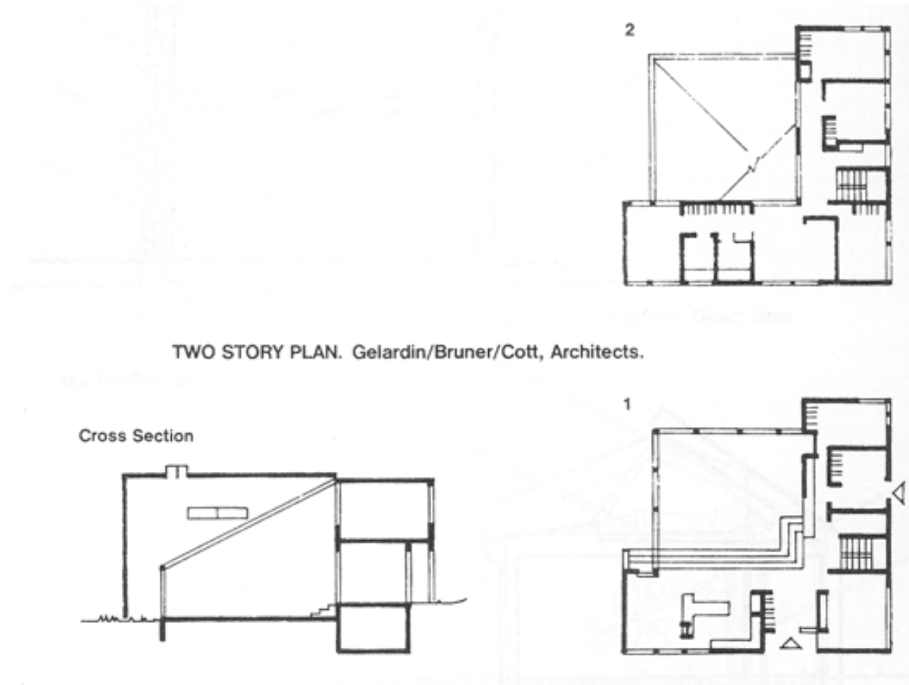
FIG. 20b. In lieu of or in addition to, orienting the majority of living areas for direct solar collection, a single "sunspace" can be used to fully maximize solar collection. Typical examples are attached greenhouses and internal glazed-roofed atria.
